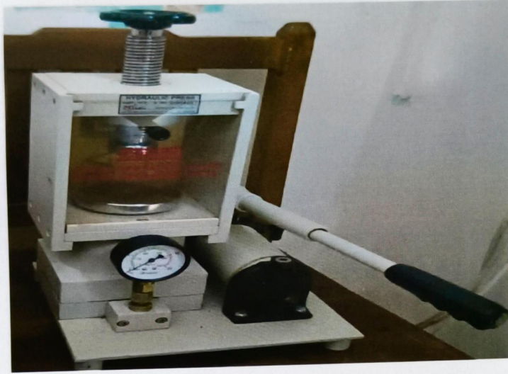
FTIR KBr- PELLET MAKER
