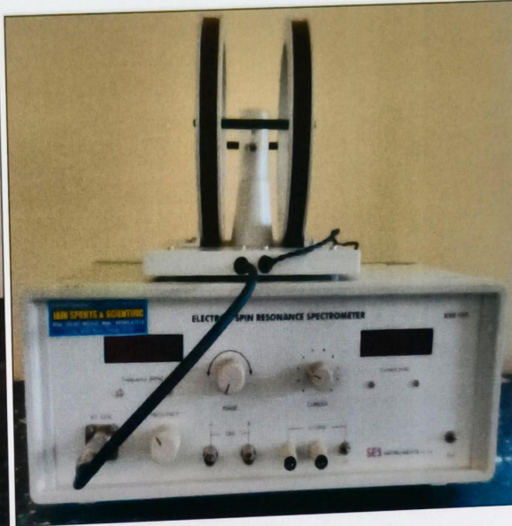
ELECTRONIC SPIN RESONANCE SPECTROMETER
